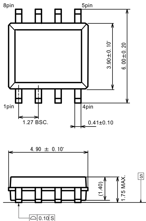
8-pin plastic SOP
